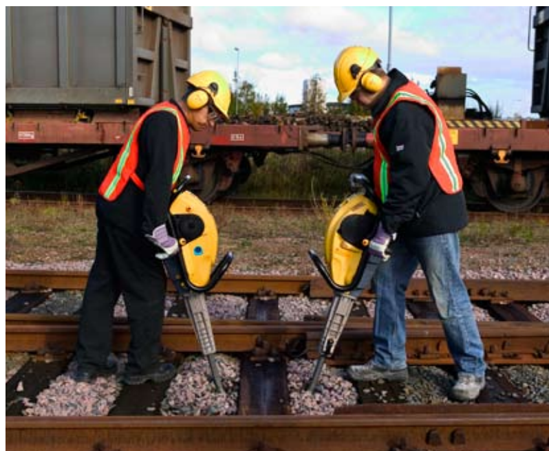
Tie tamping
