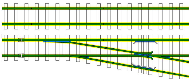
Drawing of grinding areas for MP6
